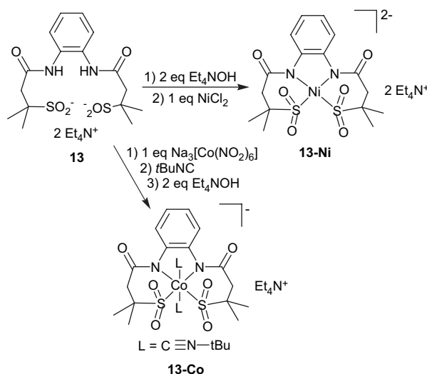
Scheme 6. Metalation of the bis-sulfinate with Ni(II) and Co(III).
