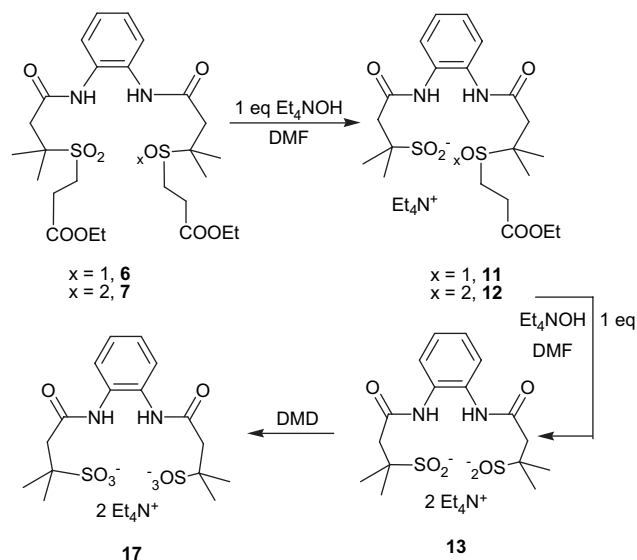
Scheme 3. Synthesis of mixed sulfonates/sulfoxide and sulfone, bis-sulfinate, and bis-sulfonate via a combination of retro-Michael reactions and DMD oxidation.
