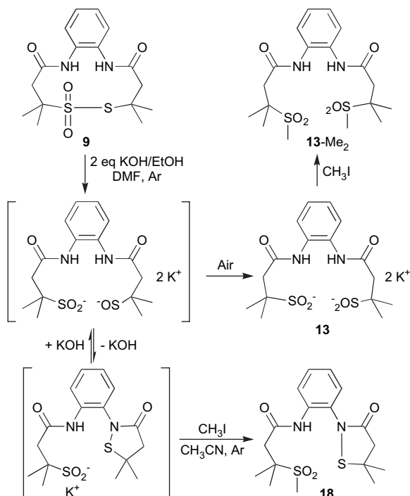
Scheme 5. Products derived from the ring-opening of the thiosulfonate.
