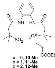
Scheme 4. Structures of the sulfones.
