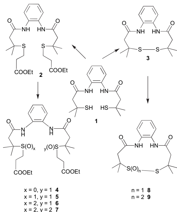
Scheme 1. Structures of the neutral sulfur compounds.
