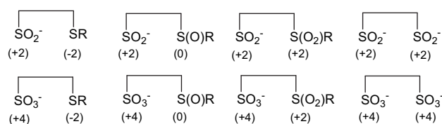
Scheme 7. Formal oxidation states of the different sulfinate and sulfonates synthesized.
