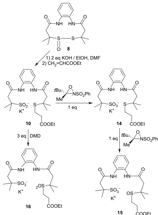
Scheme 2. Synthesis of the sulfinate/thioether and of mixed sulfonates/thioether, sulfoxide, and sulfone via a combination of ring-opening of the thiosulfinate and selective oxidations.
